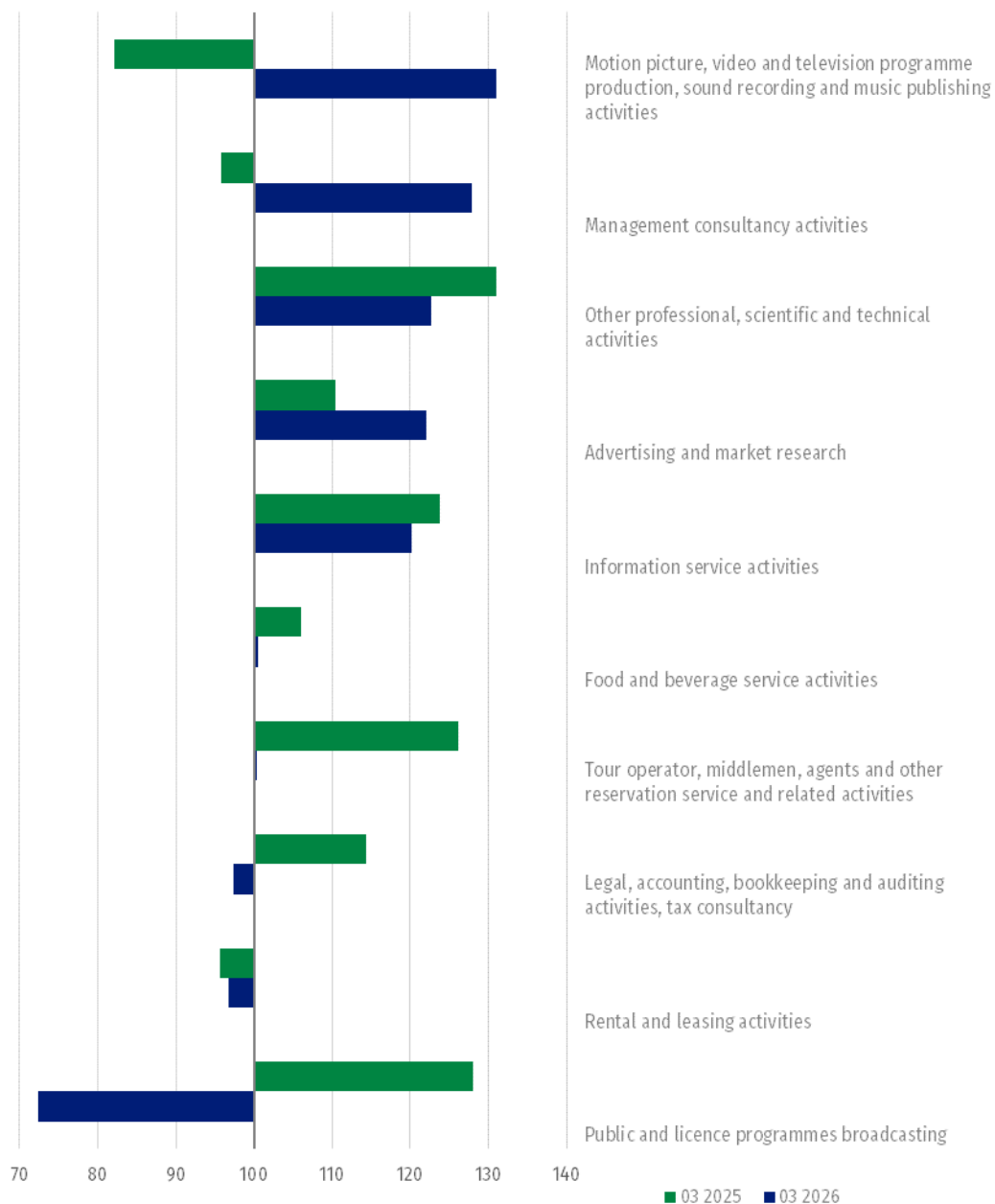
Chart 3. Dynamics of services production in selected PKD 2007 divisions (constant prices; corresponding month of the previous year=100; unadjusted data) 2
