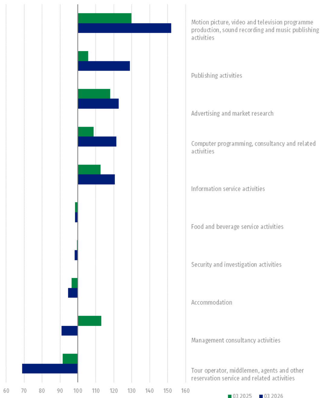
Chart 4. Dynamics of services production in selected PKD 2007 divisions (constant prices; previous month=100; unadjusted data) 2
